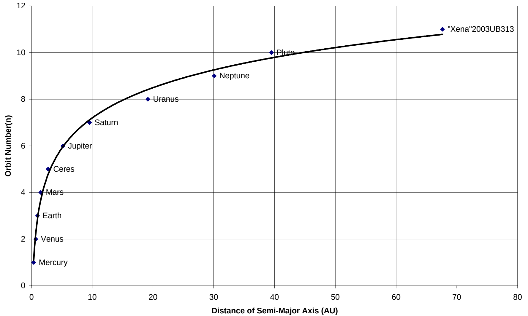
Figure: planetary and pseudo-planetary orbits
